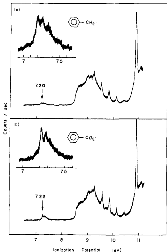
Figure 5. Pyrolysis spectra of 2-phenylethyl nitrite. NO and \text{CH}_2\text{O} are at 9–10 and 10.88 eV, respectively. The small peak at 9.0 eV is the HeI \beta ionization of \text{CH}_2\text{O} : (a) the first band of benzyl radical; (b) the first band of benzyl- \alpha - d_2 radical.
